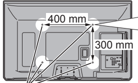
Holes for wall-hanging bracket installation
